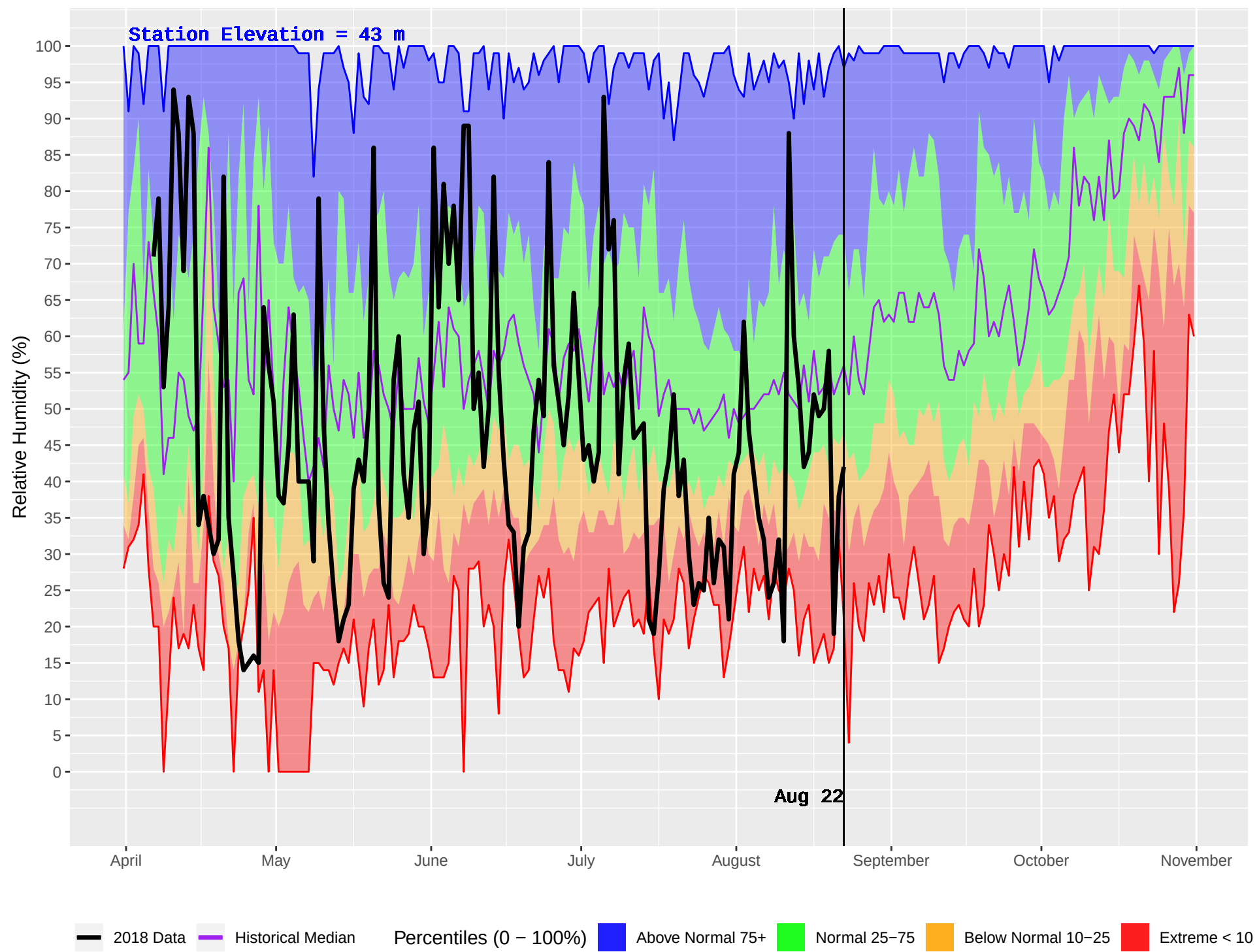
TOBA CAMP (75) : Historical (1970–2016) and Current (2018) Daily Relative Humidity
