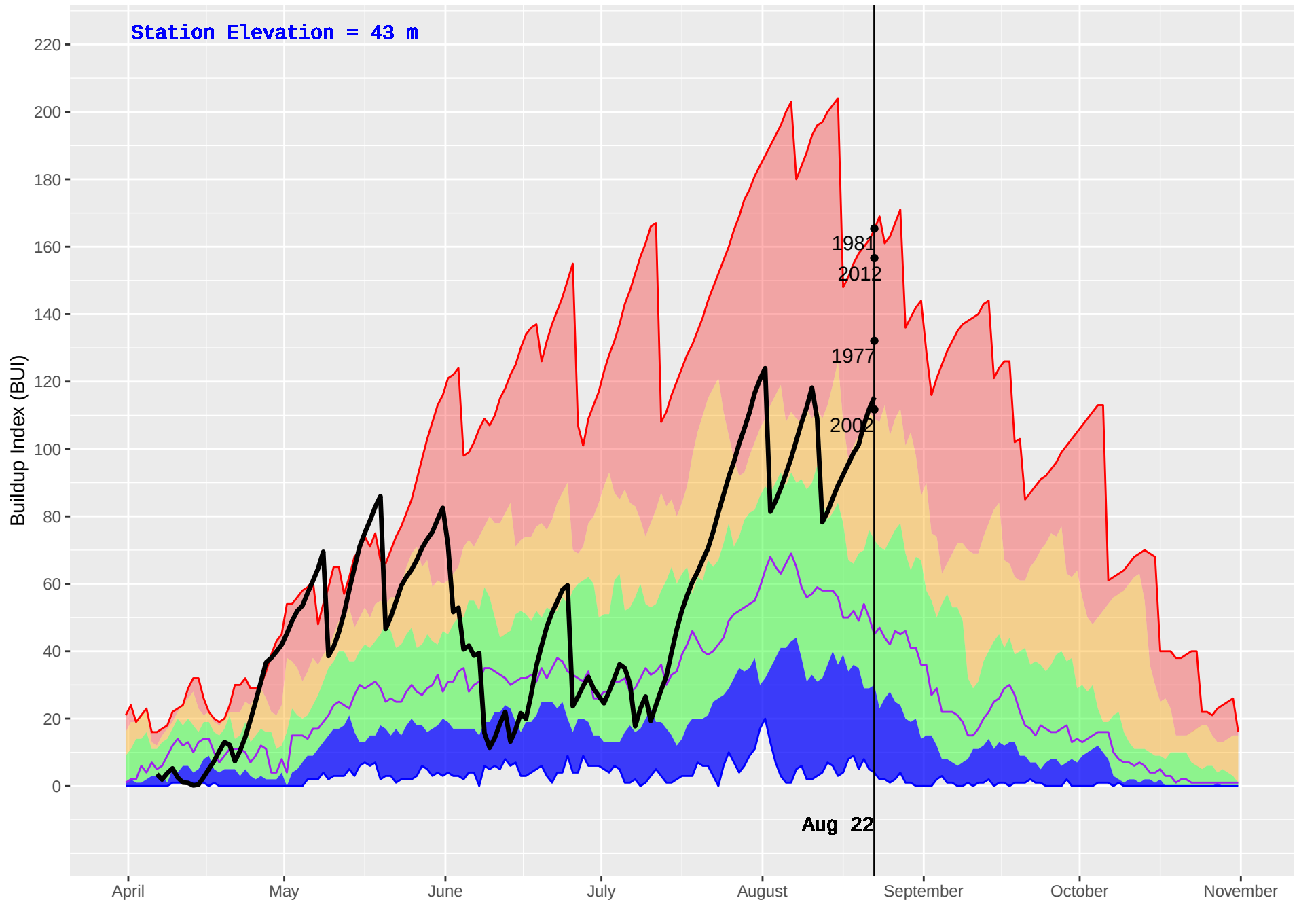
TOBA CAMP (75) : Historical (1970–2016) and Current (2018) Daily Buildup Index (BUI)
